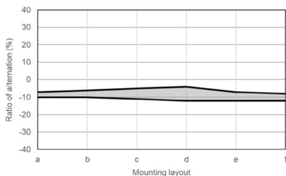
Alteration of release voltage
