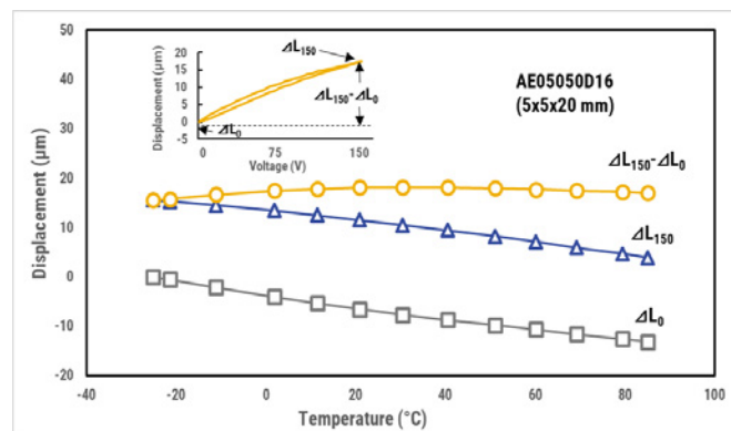
Figure 5 - Temperature vs. Displacement
