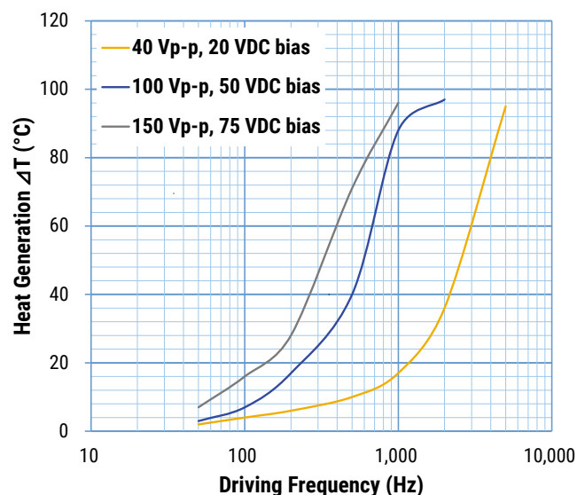
Figure 7 - Heat Generation vs. Drive Frequency - 2 Model: AL0505D16KF Temperature measurement: 5 minutes later from operation
