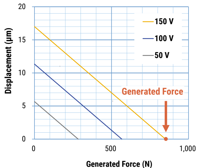
Figure 2 - Generated Force vs. Displacement of AL0505D18KF in Driving Voltage
