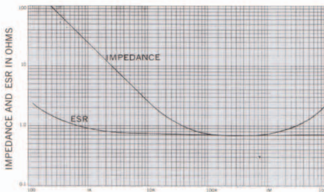
FIG. 6b 4.7 uf — 20V FREQUENCY IN HERTZ
