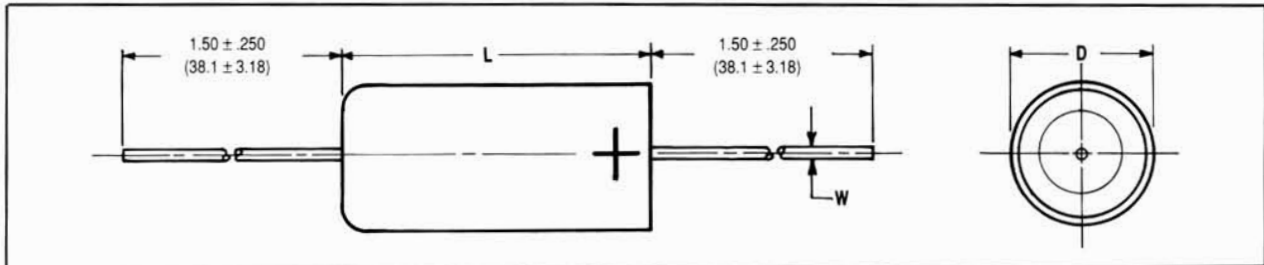
DIMENSIONS—INCHES & (MILLIMETERS)
