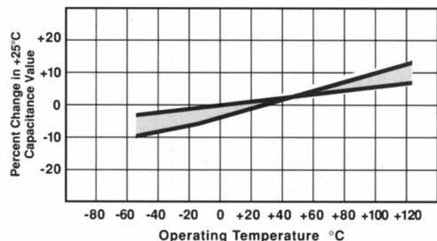
FIG. 1 TYPICAL VARIATION OF CAPACITANCE WITH TEMPERATURE
